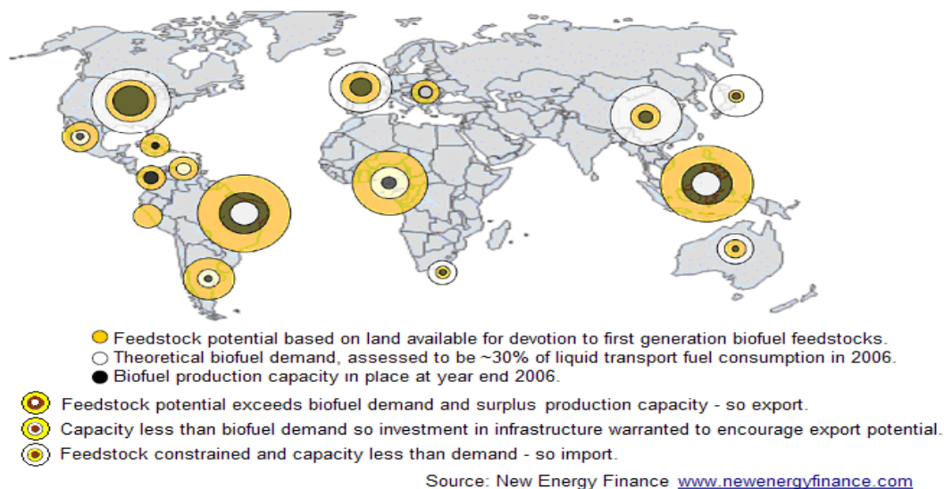
Figure 1. Indication of first generation biofuel feed stock potentials, theoretical biofuel demands and production capacities in place at end of 2006 for selected world regions. (Areas of circles depict approximate comparative scales).
